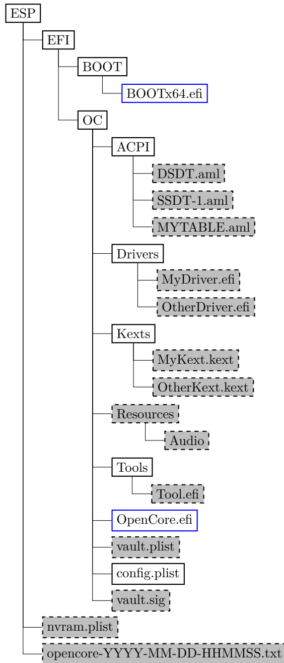
Figure 1. Directory Structure
