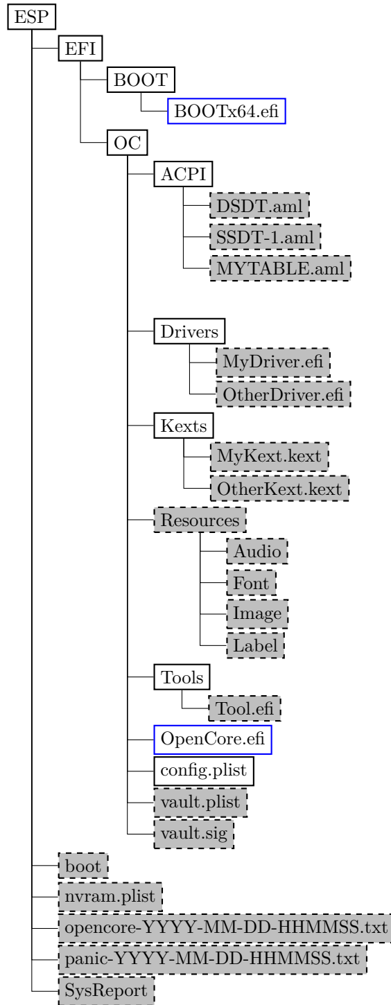
Figure 1. Directory Structure
